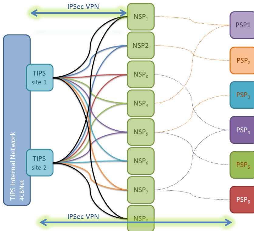
FIGURE 1 – TOWER OF BABEL CONNECTIVITY MODEL
