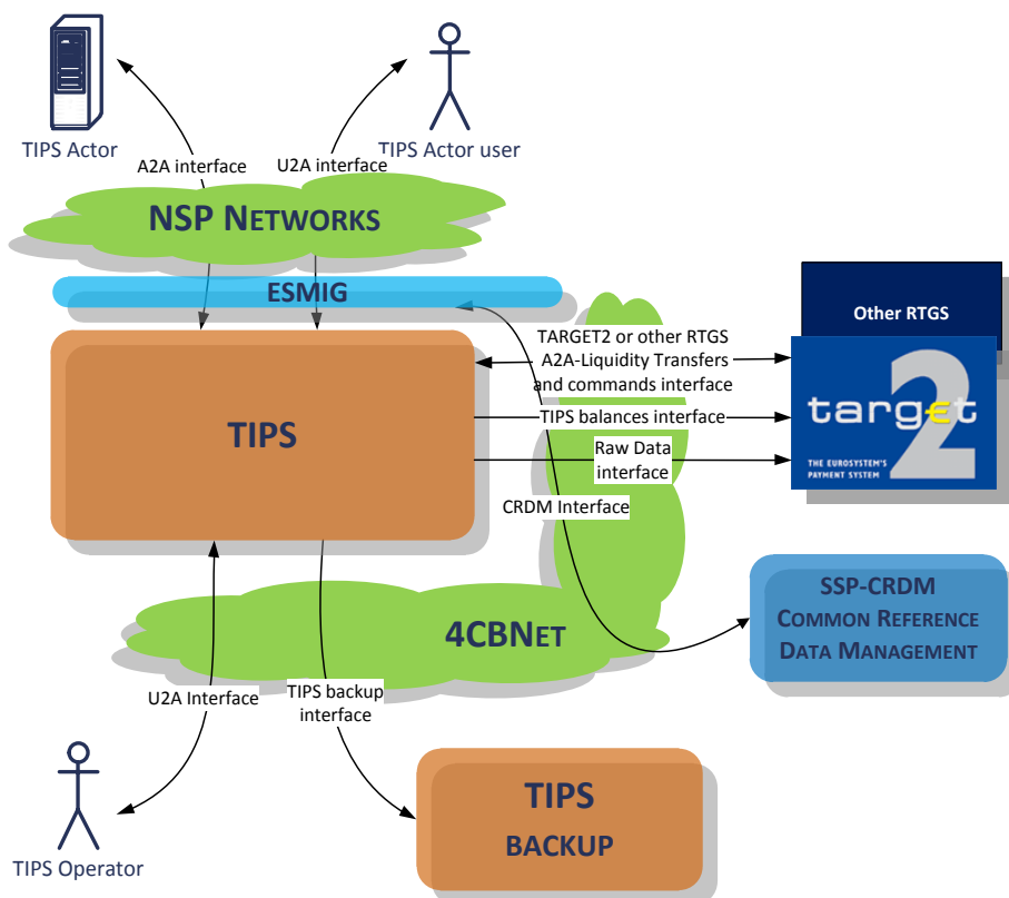
FIGURE 2 – TIPS OVERALL DIAGRAM AND TYPES OF NETWORKS
