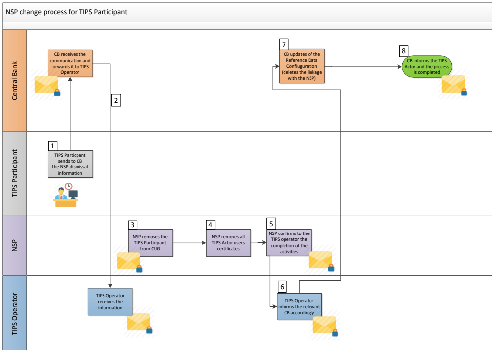
FIGURE 7 – NSP DISMISSAL FOR A TIPS PARTICIPANT
